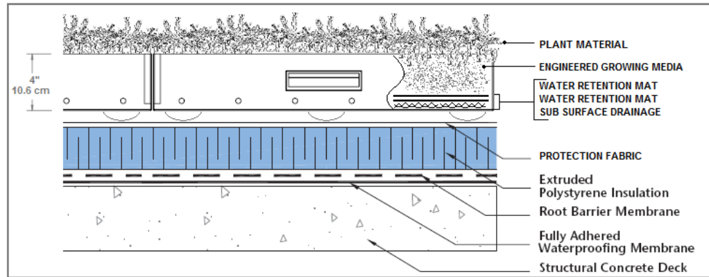
GREEN LIVING™ ROOF TRAY PROTECTED MEMBRANE APPLICATION
